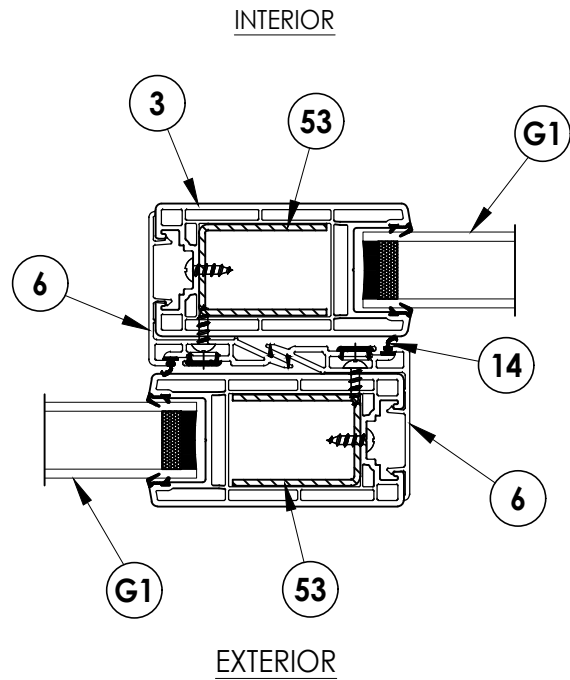
1 2 HORIZONTAL CROSS SECTION Shown w/ 2X Buck
